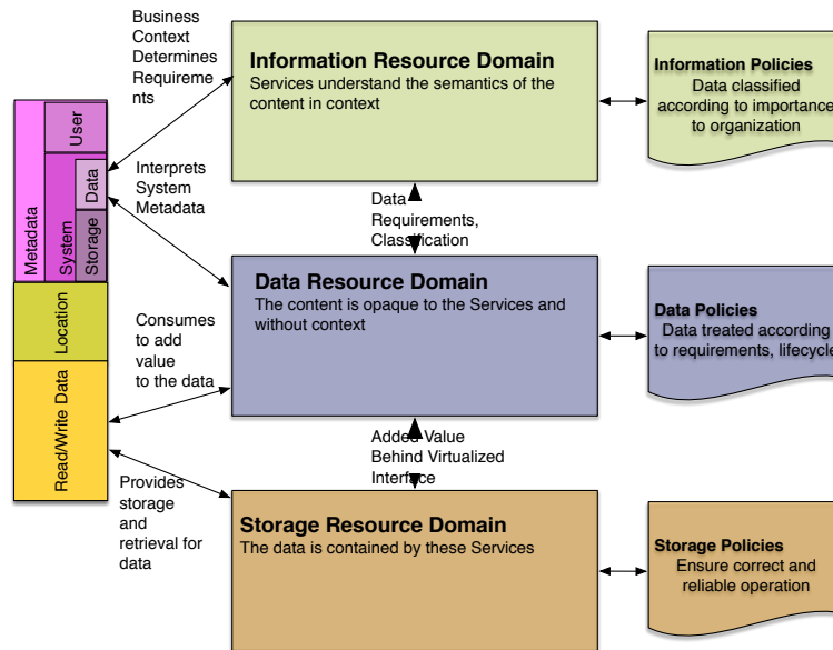
Figure 6: Resource Domain Model
