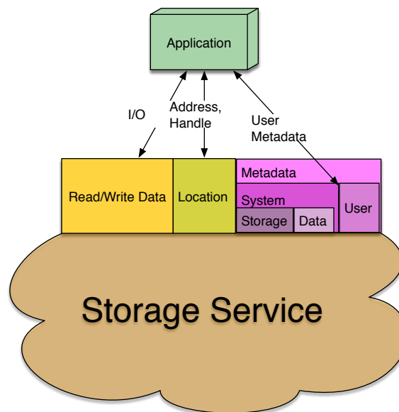
Figure 3: Storage Service use of Data Storage Interface
