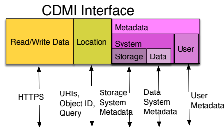
Figure 1: CDMI Data Storage Interface Standard
