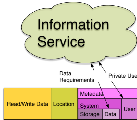
Figure 5: Information Service use of Data Storage Interface
