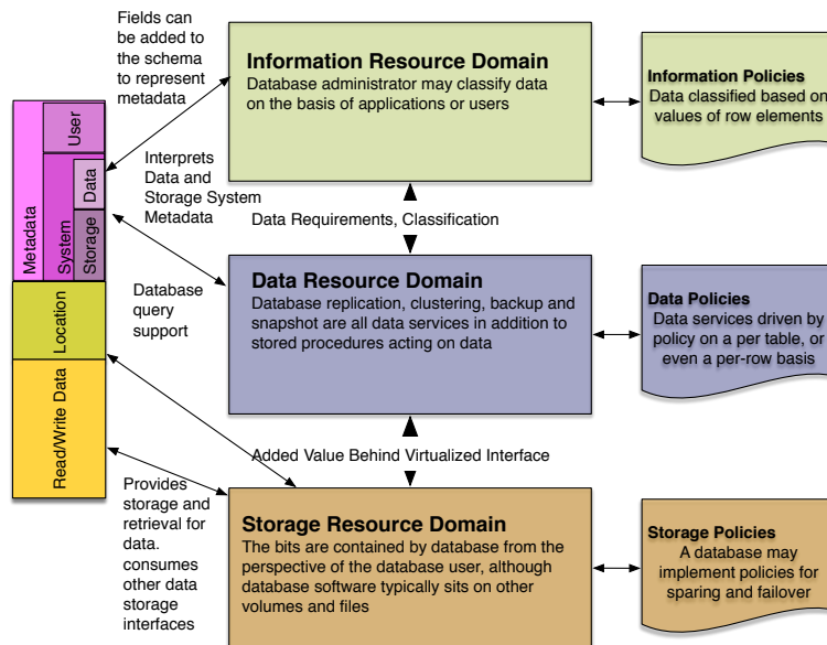
Figure 9: Resource Domain Model of an Array with Snapshot and Remote Replication
