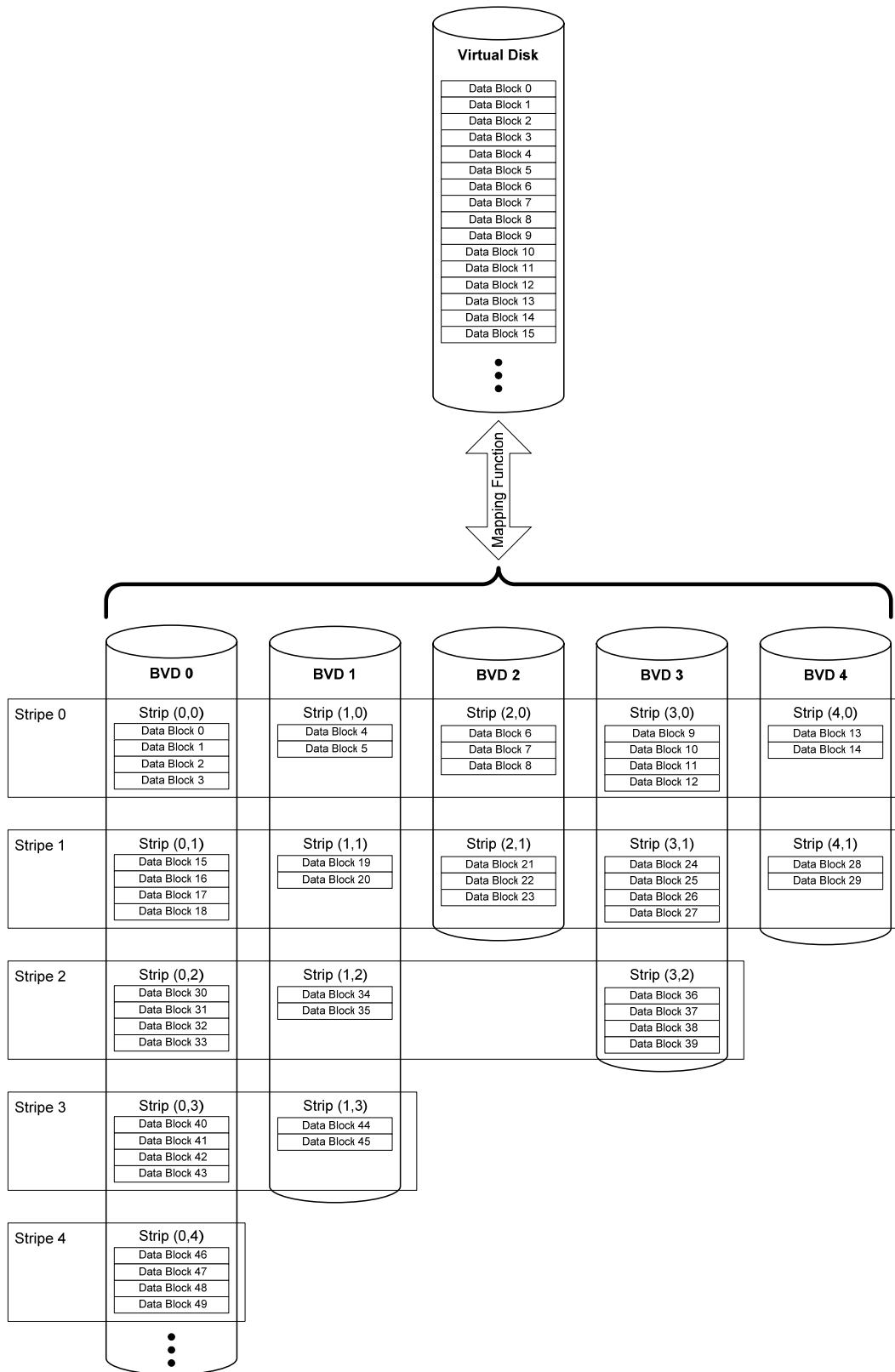
Figure 26: Spanned Secondary RAID Level (SRL=03)
